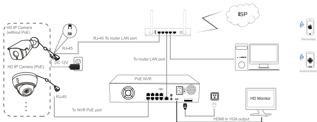
Figure 1: Working With PoE NVR
