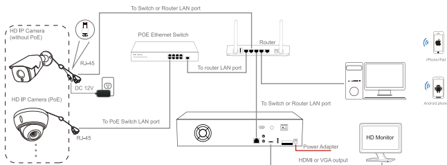
Figure 2: Working With PoE switch and NVR
